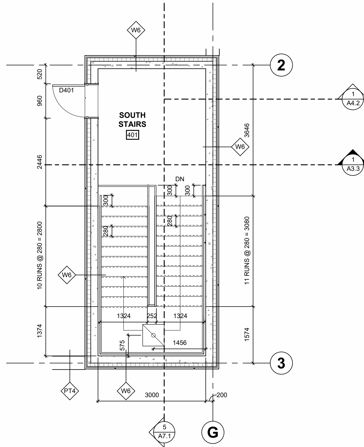
4 SOUTH STAIRS FOURTH FLOOR PLAN A7.1 SCALE = 1 : 50
