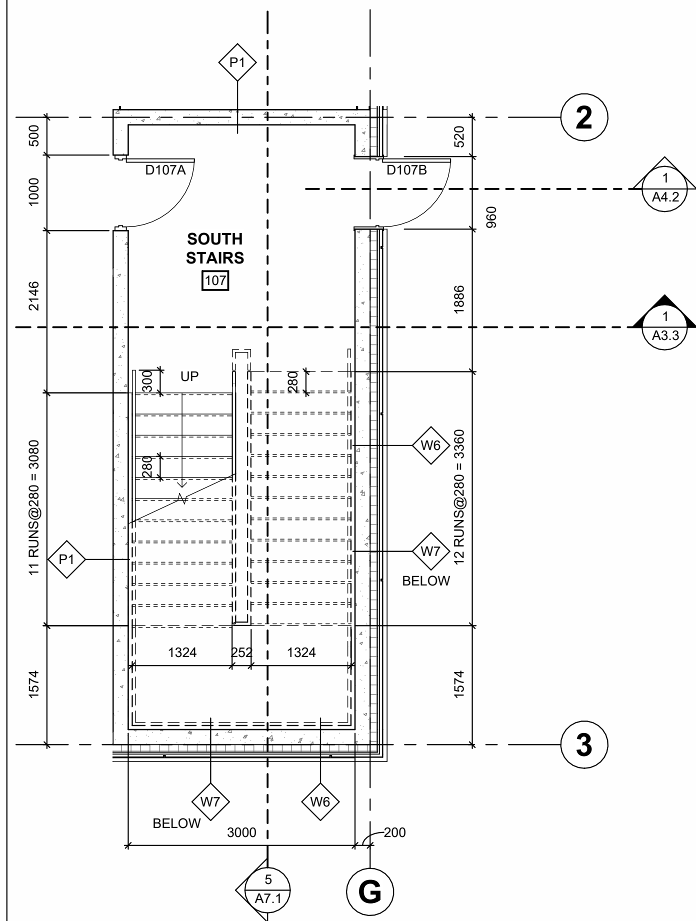
1 SOUTH STAIRS MAIN FLOOR PLAN A7.1 SCALE = 1 : 50
