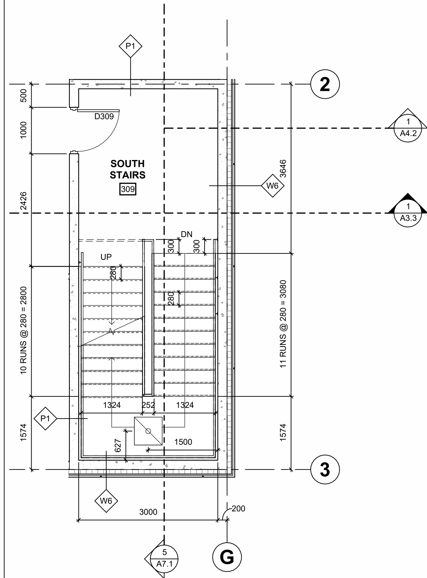
3 SOUTH STAIRS THIRD FLOOR PLAN A7.1 SCALE = 1 : 50
