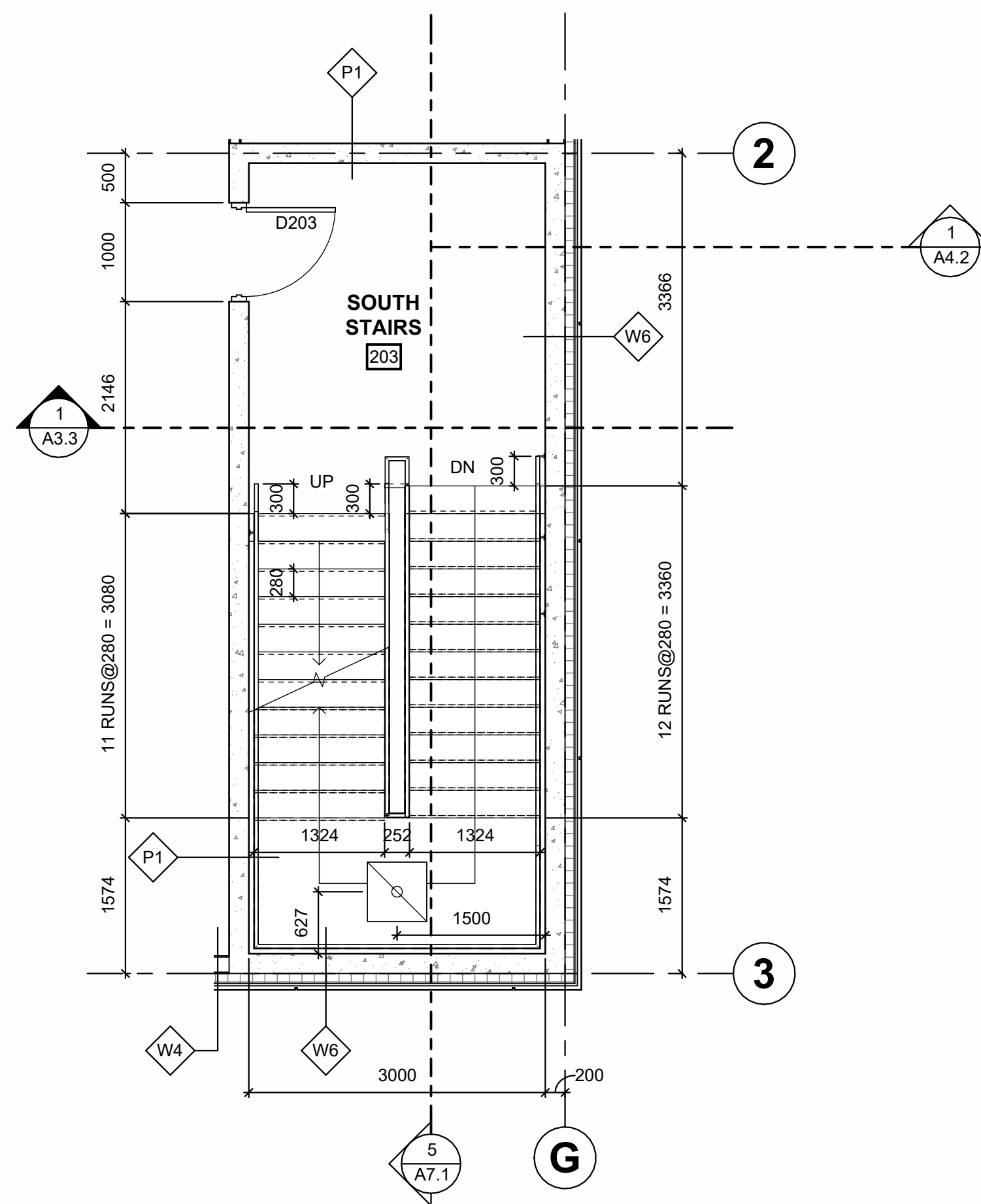
2 SOUTH STAIRS SECOND FLOOR PLAN A7.1 SCALE = 1 : 50
